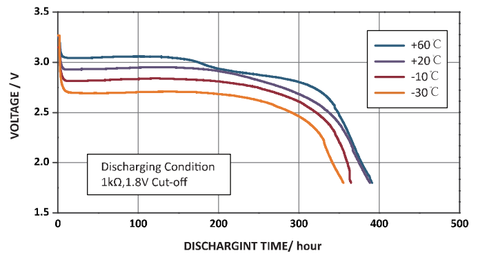
Discharging Characteristics by Temperature
