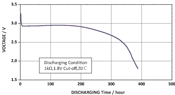
Discharging Characteristics
