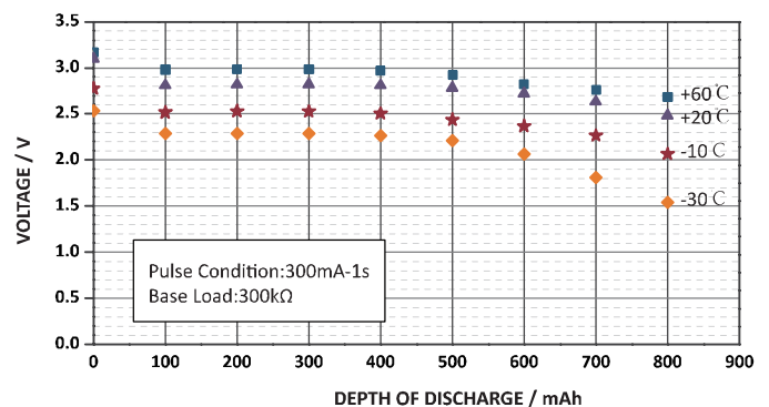
Pulse Discharging Characteristics
