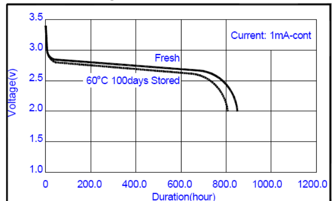
Discharge Characteristics
