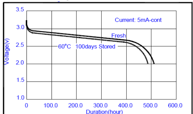
Discharge Characteristics
