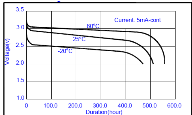
Discharge Characteristics
