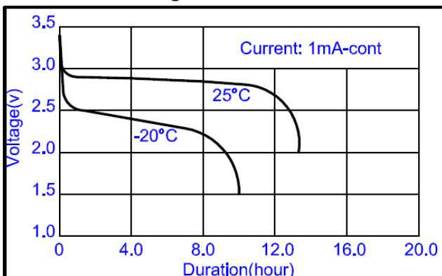
Discharge Characteristics
